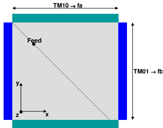
Figure 7: Nearly square patch fed on the diagonal
